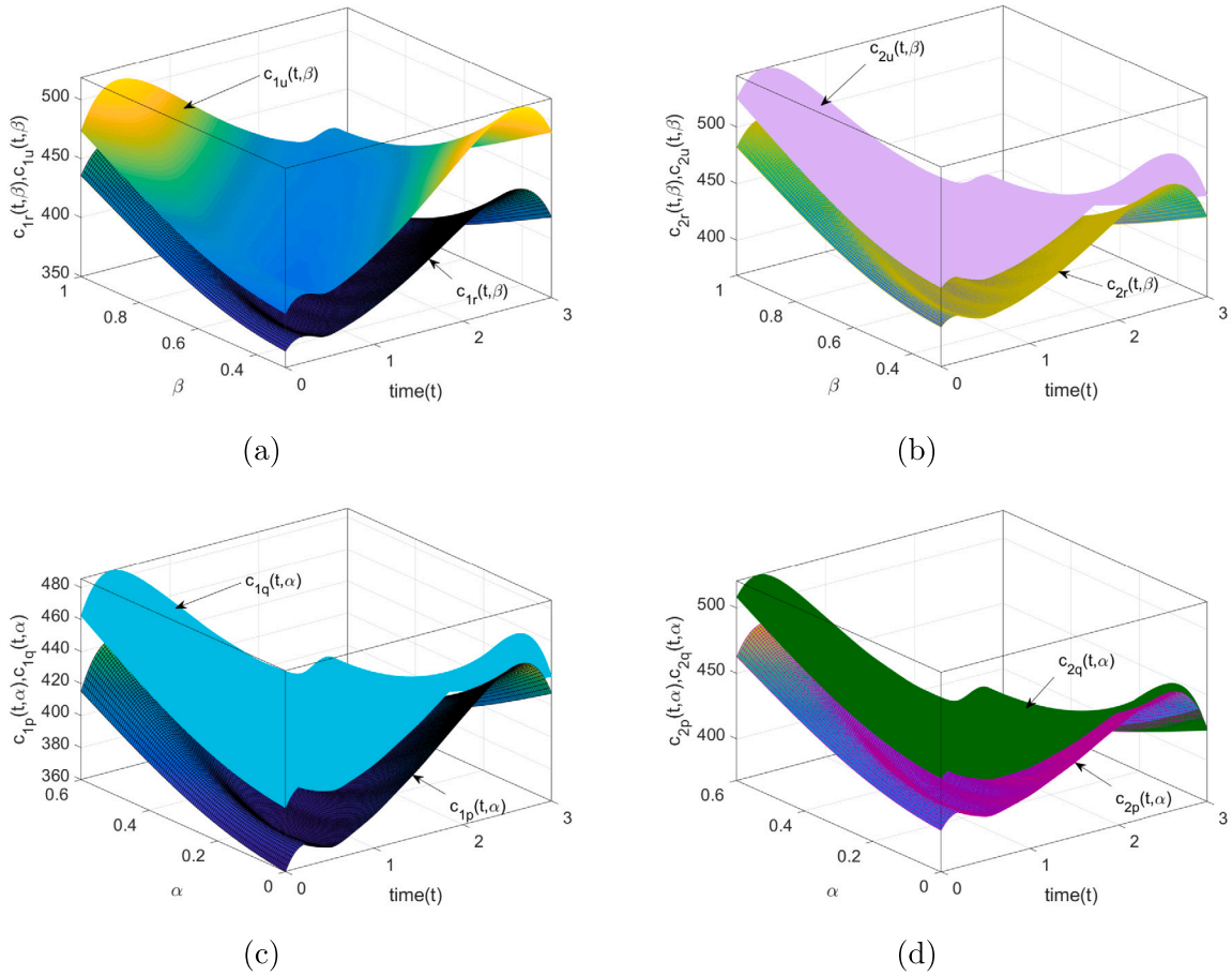
Fig. 7. 3D plot in Fig. 7(a) c_{1r}(t, \beta), c_{1u}(t, \beta) vs. time(t) vs \beta where t \in [0, 3], \beta \in [0.3, 1] ; in Fig. 7(b) c_{2r}(t, \beta), c_{2u}(t, \beta) vs. time(t) vs. \beta where t \in [0, 3], \beta \in [0.3, 1] ; in Fig. 7(c) c_{1p}(t, \alpha), c_{1q}(t, \alpha) vs. time(t) vs. \alpha where t \in [0, 3], \alpha \in [0, 0.6] ; in Fig. 7(d) c_{2p}(t, \alpha), c_{2q}(t, \alpha) vs. time(t) vs. \alpha where t \in [0, 3], \alpha \in [0, 0.6] .
